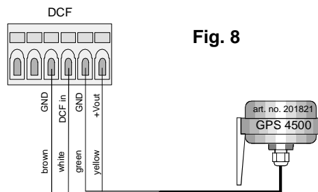
GPS receiver
